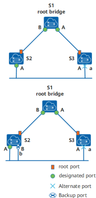
Figure12-11 Port Role Schematic
