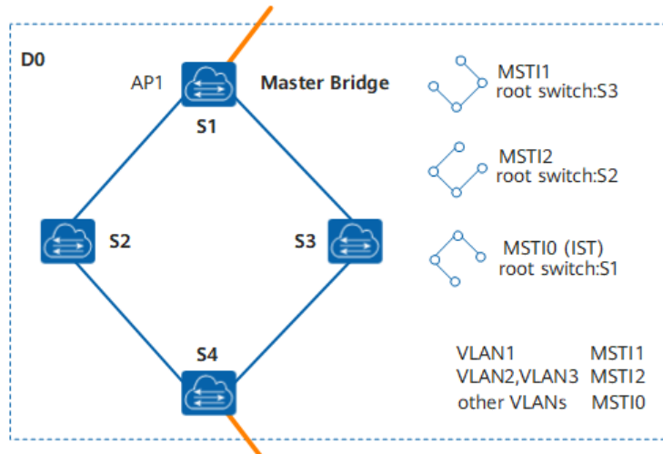
Figure12-17 Basic Concept Diagram of MST Region
