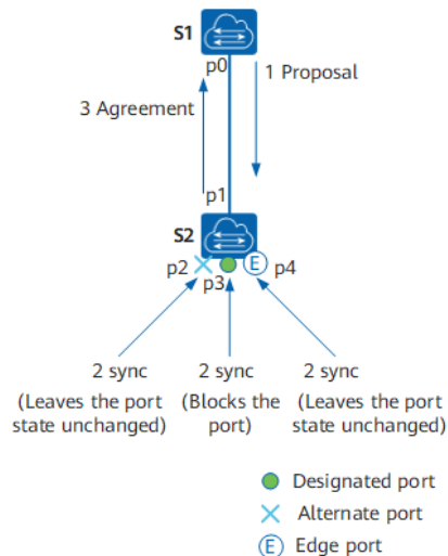
Figure12-13 Proposal/Agreement Process Diagram
